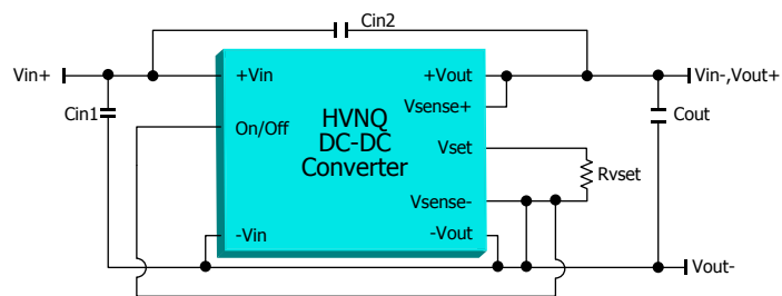
Figure D: Negative output setup
